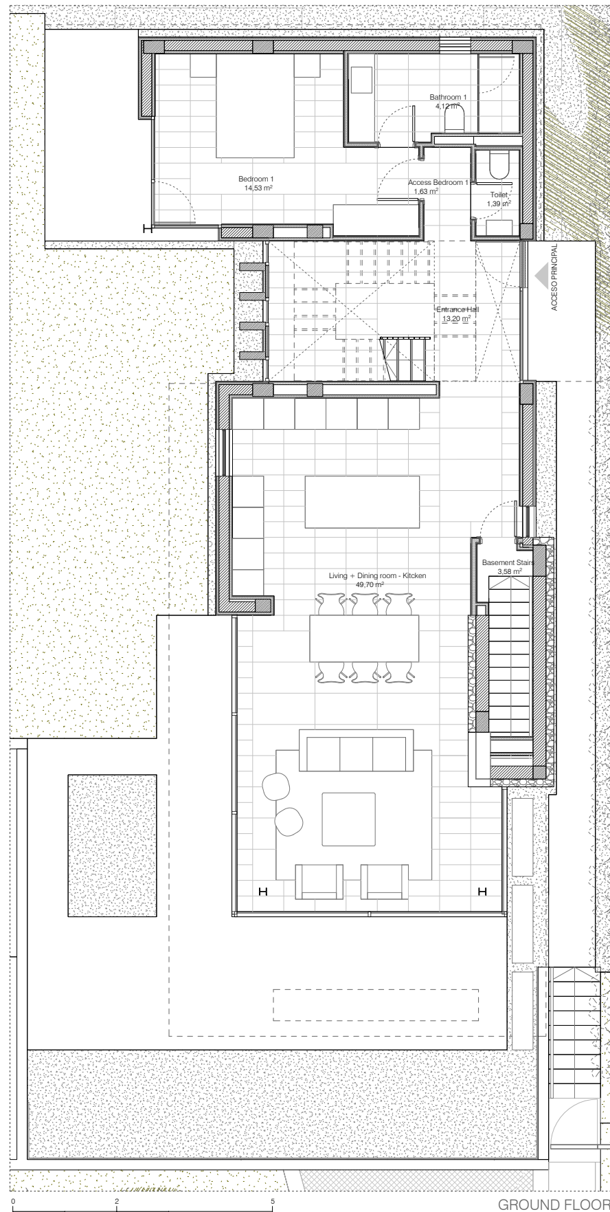
GROUND FLOOR
