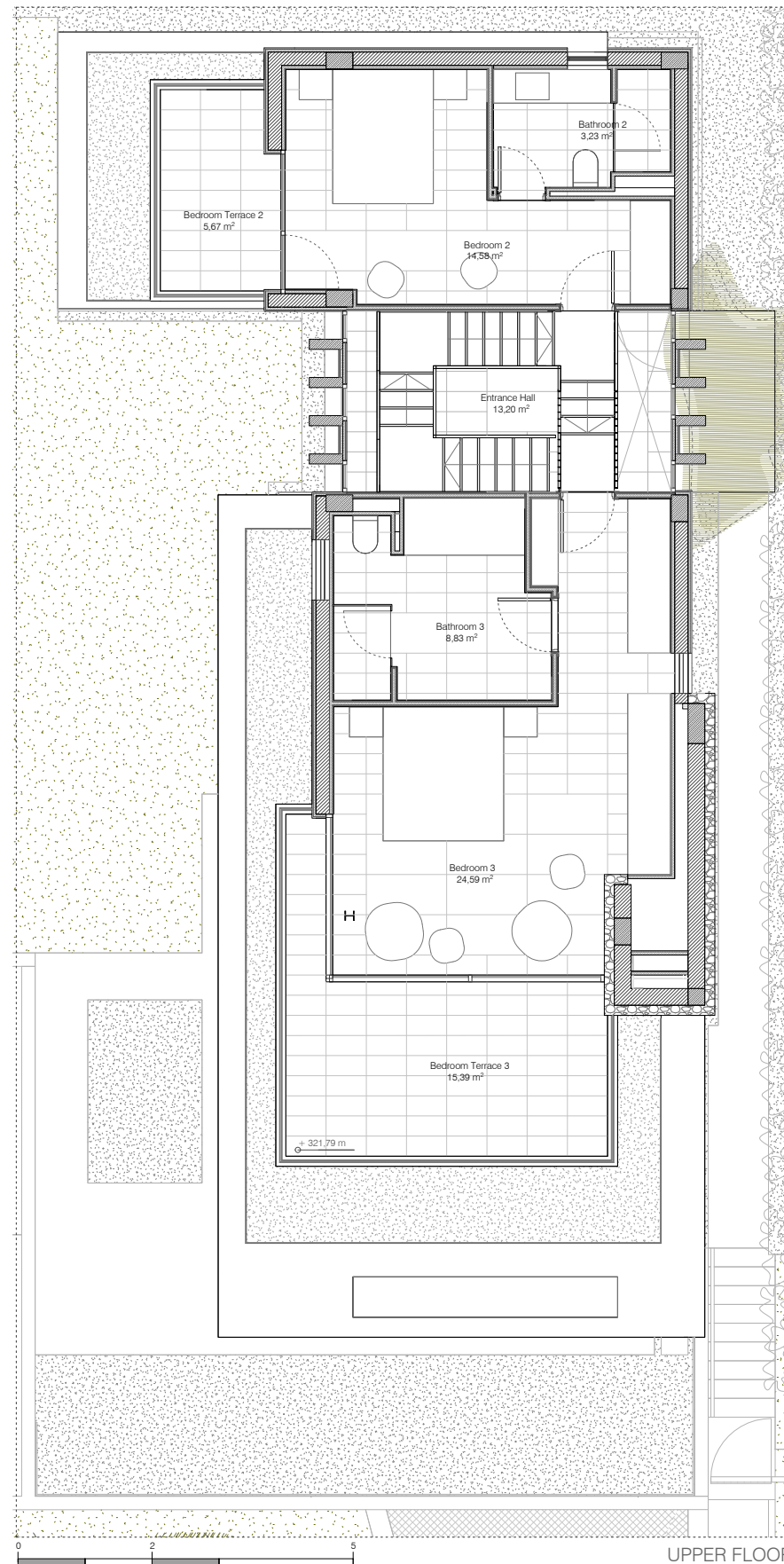
UPPER FLOOR
